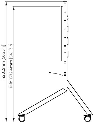
Side View Lowest Horizontal Bar Assembly
