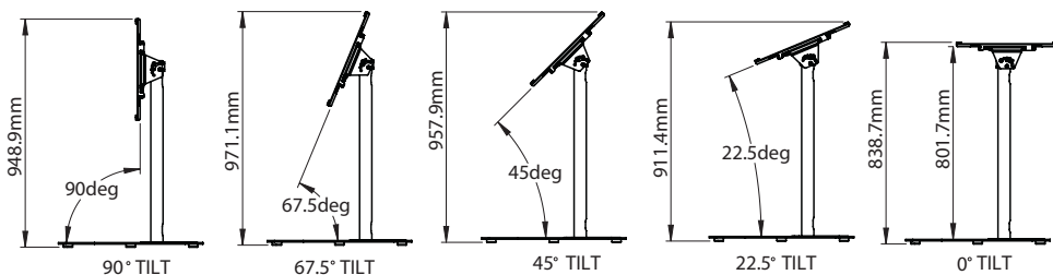
SIDE VIEW - TILT RANGE
