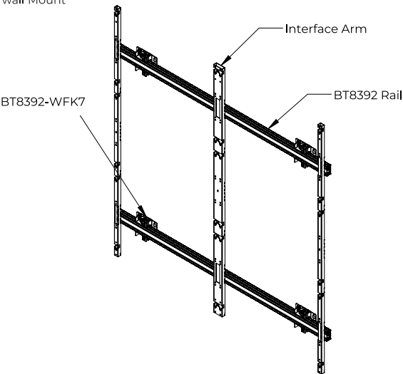
4x4 dvLED Videowall wall Mount
