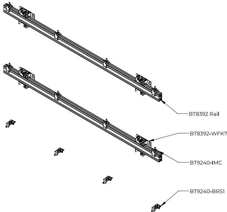
System Xpress 4x4 dvLED Videowall Mount
