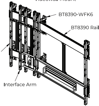
BT9343 Curved dvLED Videowall Mount
