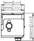
Side View with BT8390 Rail (Centre depth)
