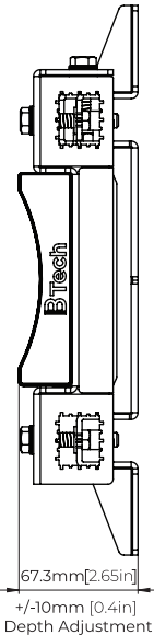
Side View with BT8390 Rail (Centre depth)
