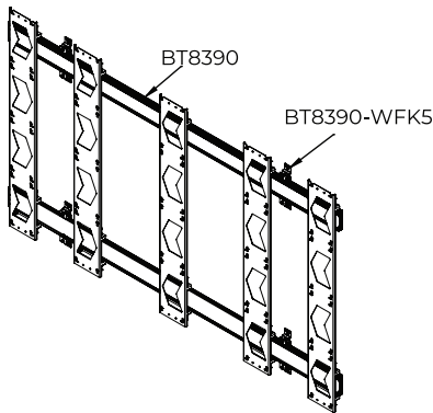
dvLED RM Videowall Wall Mount
