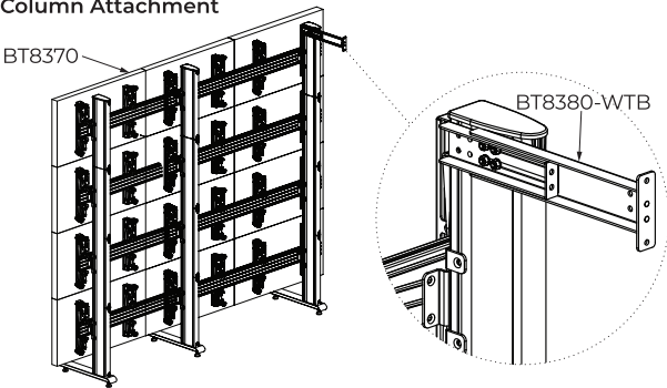
Column Attachment
