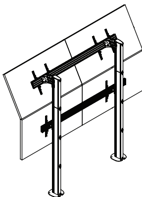
Bolt Down Videowall Stand
