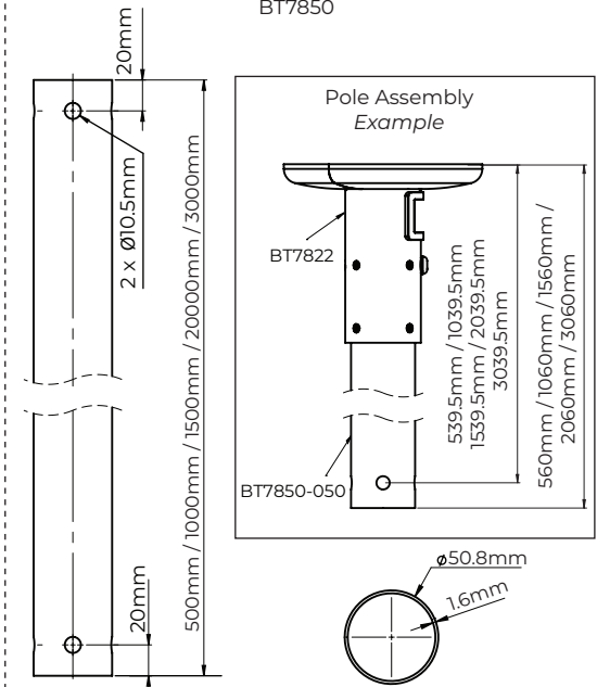
Extension Pole BT7850
