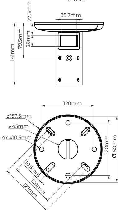
Ceiling Mount BT7822
