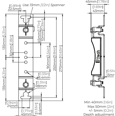
Wall Bracket - BT8390-WFK5
