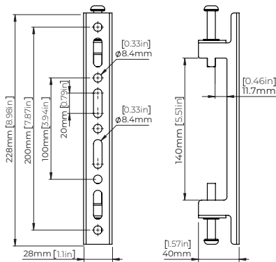
BT8390-VESA400F Fixed VESA 400mm Interface Arms
