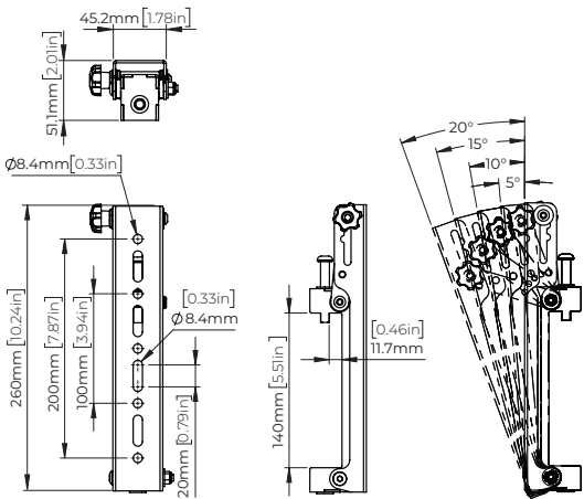
BT8390-VESA200T VESA 200mm Interface Arms with Tilt
