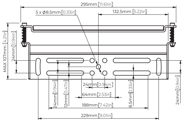
Wall Plate
