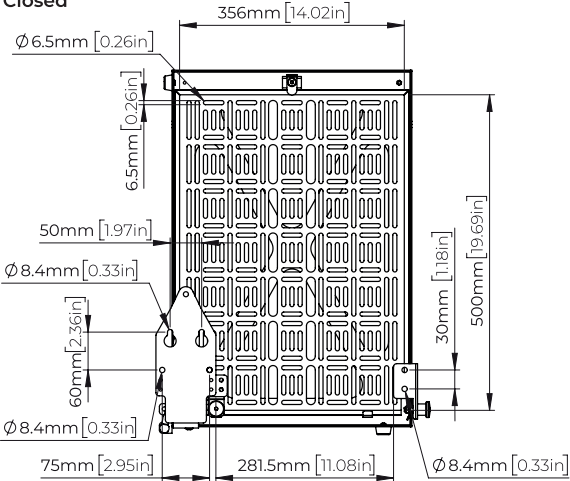
Front View - Closed
