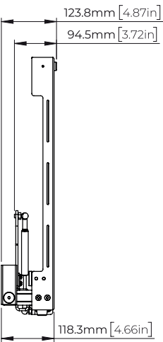
Side View - Closed
