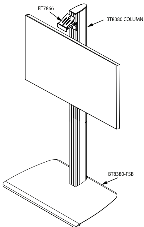
COLUMN INSTALLATION
