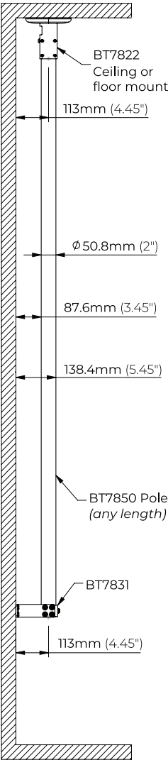
Ceiling-To-Wall Mounting Position
