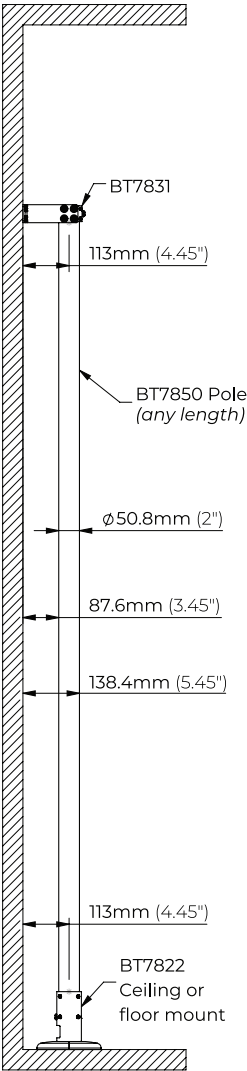
Floor-To-Wall Mounting Position
