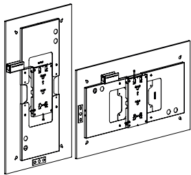
BT7611-SAM32 Wall Mount with Tilt
