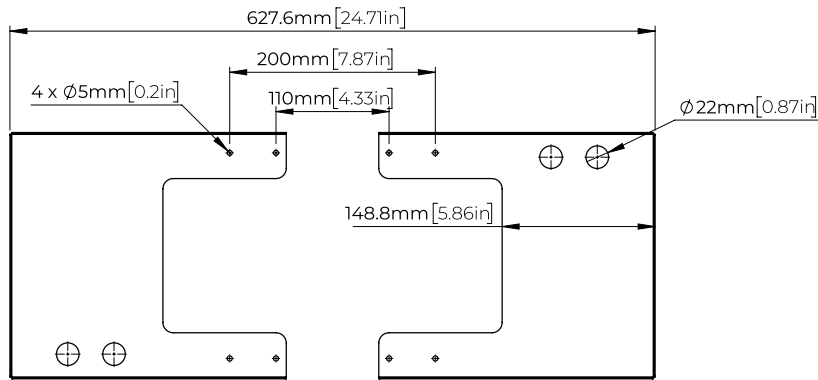
POSITION B - Covering of Battery Compartment and Ports
