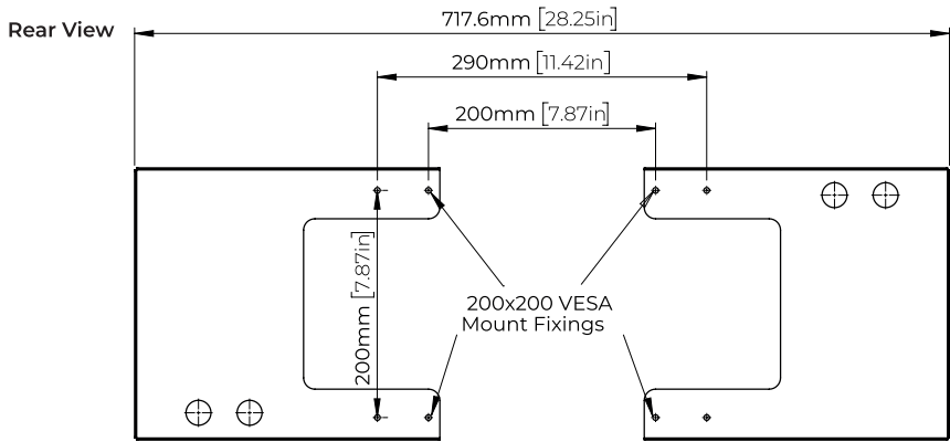
POSITION A - Covering of Battery Compartment Ports and Buttons
