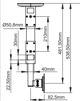
BT7553-050
