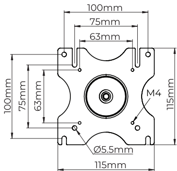
Interface Plate
