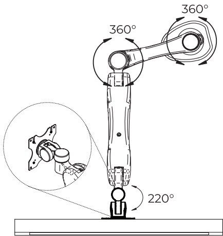
Screen Rotation
