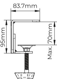
Desk Clamp
