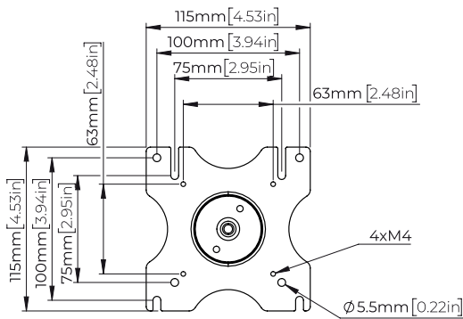
Interface Plate
