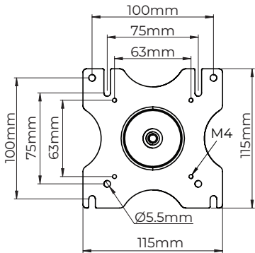
Interface Plate
