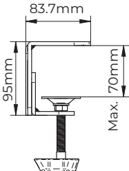
Desk Clamp
