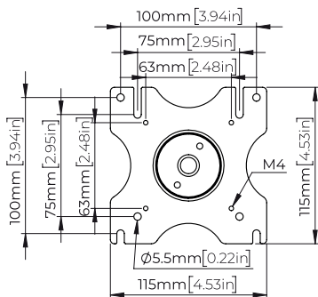
Interface Plate
