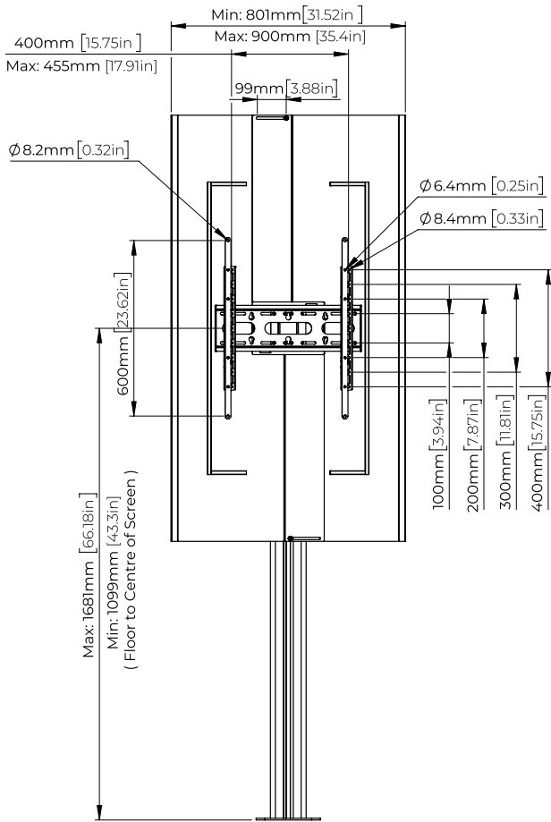
Front View
