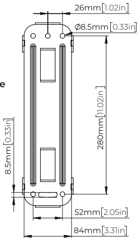
Wall Plate
