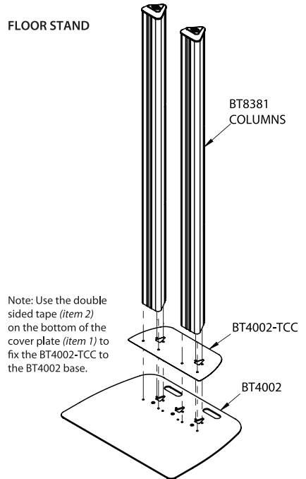
EXAMPLE INSTALLATION
