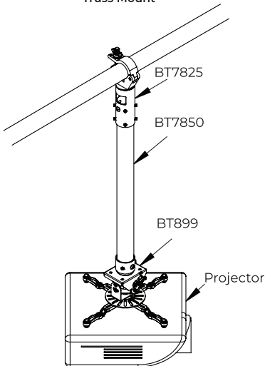
Truss Mount
