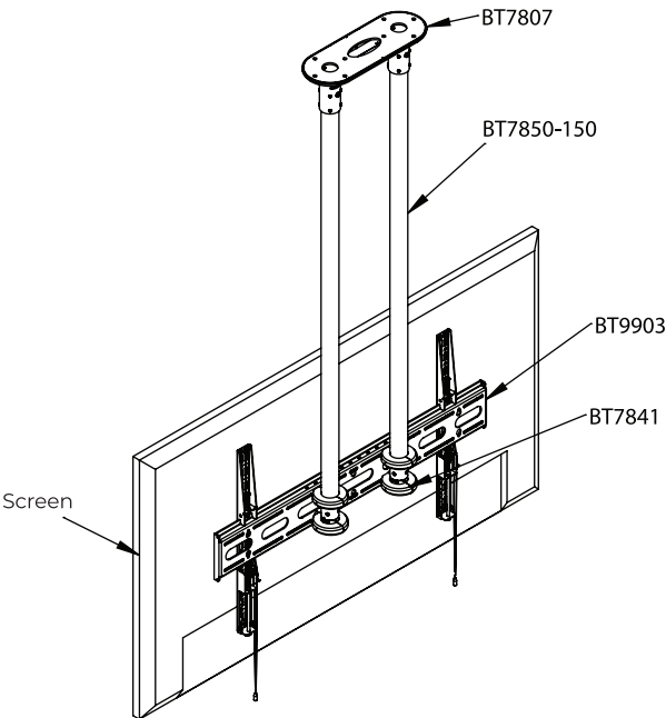
Typical Pole Installation for the BT9903
